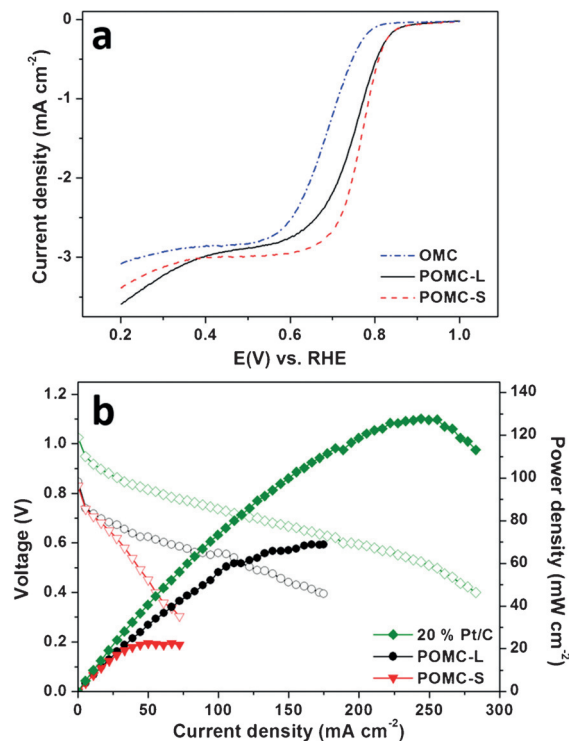
Figure 2. a) LSV polarization curves of the catalysts. b) Polarization curves of MEAs at 60°C; open and closed symbols correspond to cell voltage and power density, respectively.
